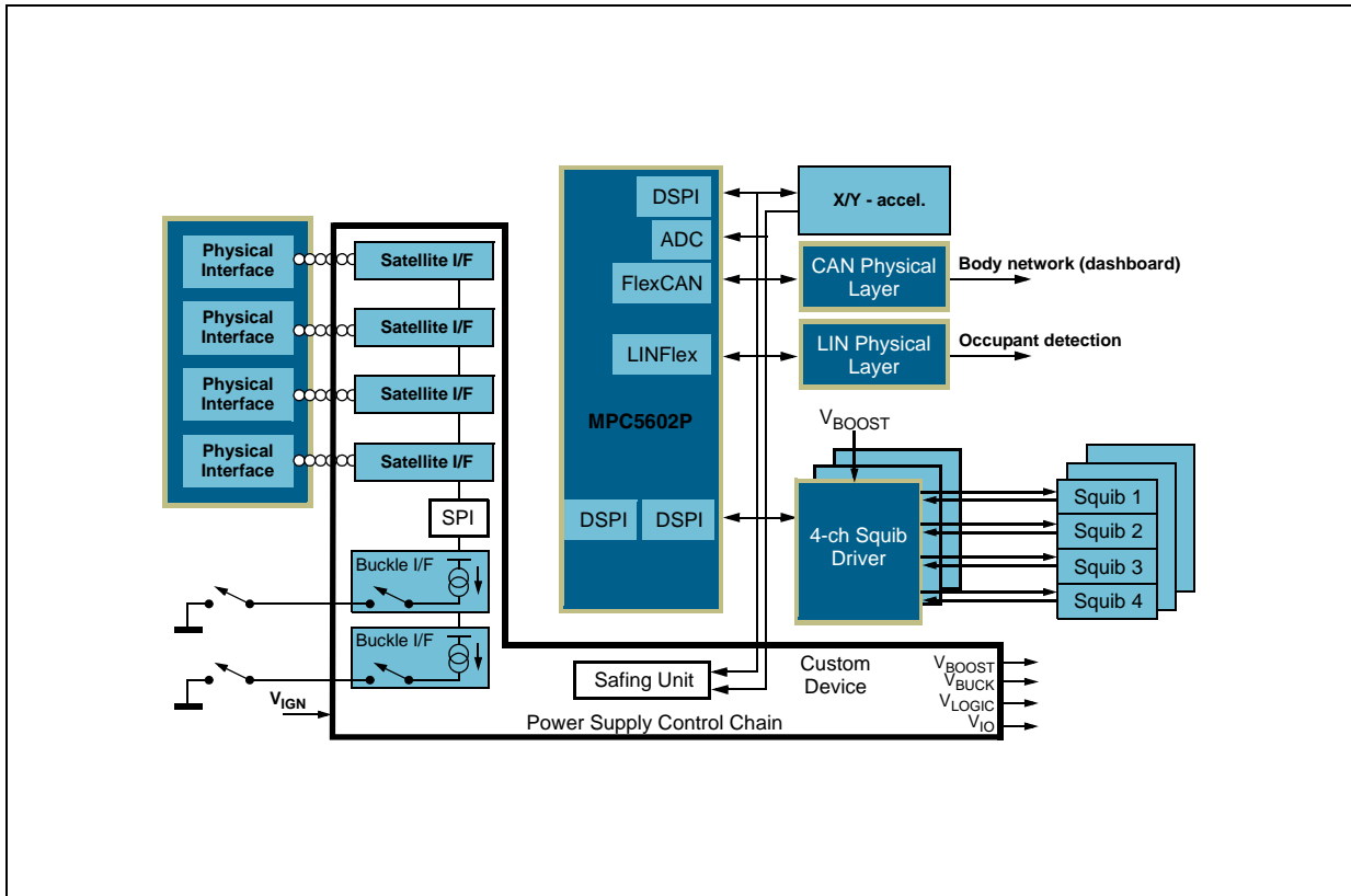
Figure 3. Airbag application
